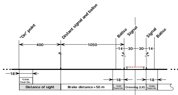
Fig.6. Plan of the existing crossing. Distances are in meters.
