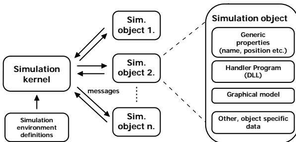
Fig.2.Simulation architecture
