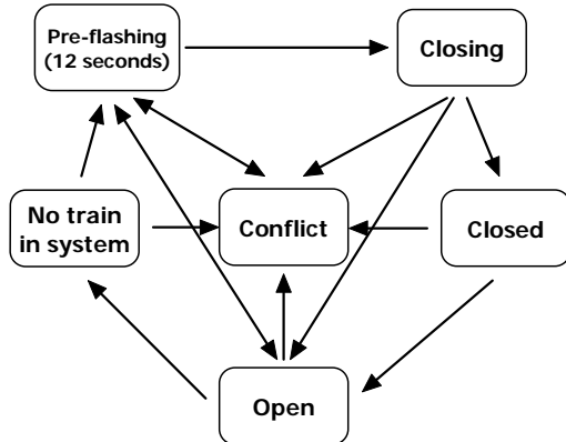
Fig.5. Graph of the level crossing's control object
