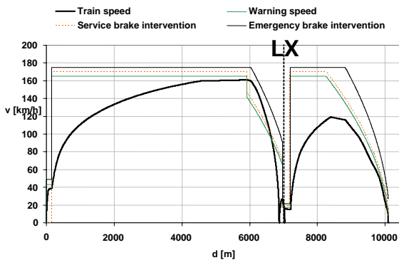
Fig.8. Distance-speed diagram of a test run on the variant “c”.
