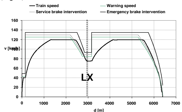
Fig.7. Distance-speed diagram of a case 2. test run on the original variant.
